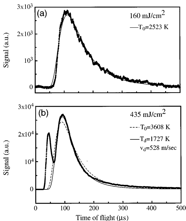
FIG. 2. (a) Time-of-flight distribution below the ablation threshold ( 160 \text{ mJ/cm}^2 ). Continuous curve: “half range” Maxwellian fit. (b) Distribution above the ablation threshold. Dashed curve: “half range” Maxwellian. Continuous curve: drifted Maxwellian.
