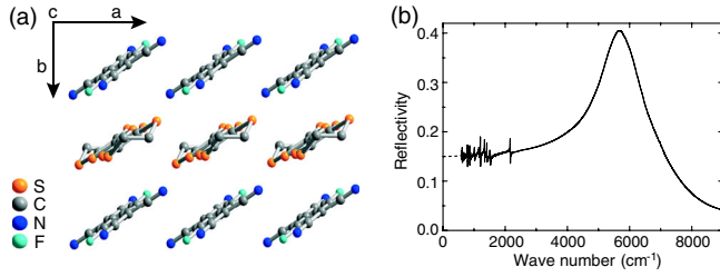
FIG. 1 (color online). (a) The crystal structure of one-dimensional organic salt ET-F 2 TCNQ (yellow, ET; blue, F 2 TCNQ). (b) Static reflectivity of the compound with electric field parallel to crystallographic a axis (along the ET chain).
