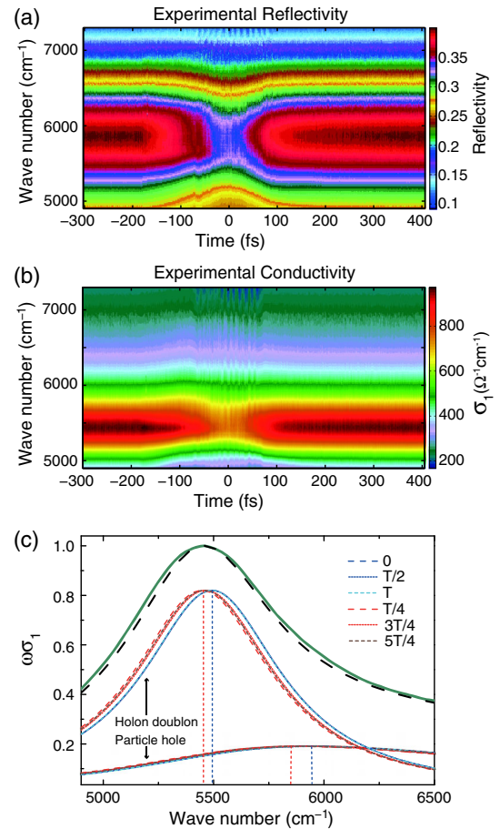
FIG. 4 (color online). (a) Frequency-resolved reflectivity as a function of pump-probe delay time. (b) Corresponding optical conductivity extracted from reflectivity using the KK variational dielectric fit function. (c) Normalized equilibrium optical conductivity (green) of ET-F 2 TCNQ at room temperature with model fit (dashed black). Below are the fitted contributions from the HD and PH continuum, individually normalized at various times along the pump electric field cycle of time period T .
