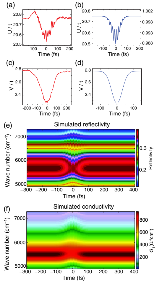
FIG. 5 (color online). (a),(c) Time dependence of effective Hubbard correlation term U/t and V/t , respectively, extracted from fits. (b) and (d) Assumed U/t and V/t variation, respectively, over time for numerical simulation, similar to one obtained experimentally. (e) Simulated reflectivity obtained via two-time current-current correlation function calculations of an effective strong-coupling model. (f) Corresponding simulated conductivity from the calculations.
