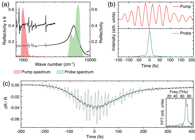
FIG. 3 (color online). (a) (red) Spectrum of the midinfrared excitation pulses centered at 1000\text{ cm}^{-1} ( 10\text{ }\mu\text{m} wavelength) resonant to the ET molecular vibration mode (blue). The sample reflectivity in direction perpendicular to the a axis is shown in gray. (green) The spectrum of the near-infrared probe beam covers the charge transfer band along the a axis. (b) (upper panel) Phase-locked electric field of the midinfrared pump pulse measured via electro-optic sampling; (lower panel) intensity profile of NIR probe pulse. (c) (green) Spectrally integrated time-dependent reflectivity changes in ET-F 2 TCNQ at a pump fluence of 0.9\text{ mJ/cm}^2 at room temperature, together with a double exponential fit of the form \text{Aerf}(t/t_d + 1)\sum_{i=1,2} A_i e^{-t/\tau_i} in dashed black. The gray solid line shows the deconvolved reflectivity changes, and the inset shows a Fourier transformation of the measured oscillations peaking at 70\text{ THz} .
