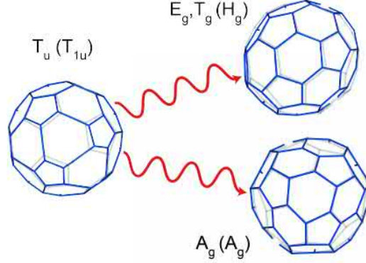
Figure 4.1: Couplings between the T_{1u}(4) mode and H_g Raman vibrations of the C_{60}^{3-} molecules. The distorted structure associated with each mode and for a 9% change of the C-C bond length are shown as blue lines while the equilibrium structure is depicted in light grey. Distorted structures have been kindly provided by Dr. Alaska Subedi.
