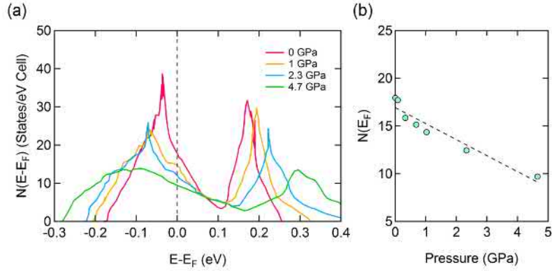
Figure 5.2: Calculated broadening of the electronic density of states of the conduction band of \text{K}_3\text{C}_{60} with external hydrostatic pressure (a) and predicted scaling at the Fermi energy (b) at room temperature. The vertical dashed line at 0 eV in panel (a) indicates the Fermi energy, while the one in panel (b) is the result of a linear fit. Figure adapted from [102].
