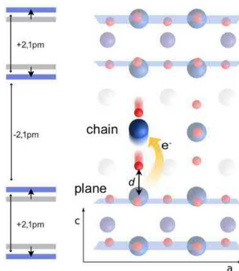
Figure 1.12: Schematic out-of-equilibrium structure of \text{YBCO}_{6.5} , reconstructed from fits of the transient scattered intensity of several peaks measured with Hard X-rays. The atomic displacements from the equilibrium structure involve a decrease in interbilayer distance, accompanied by an increase in intra bilayer distance [18, 40].
