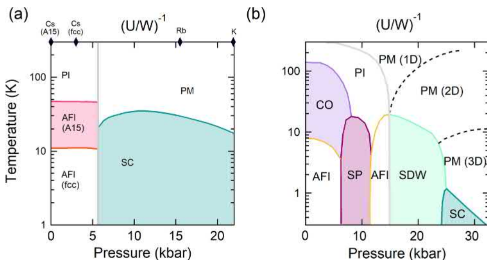
Figure 2.3: Temperature-Pressure phase diagrams for two families of organic molecular solids with different effective dimensionality. (a) The three-dimensional alkali fullerenes family A_3C_{60} with the black diamonds on the upper axis identifying the equilibrium position of different alkali dopant (adapted from [58]). (b) The one-dimensional Bechgaard salts (TMTTF)_2X (or (TMTSF)_2X ) (adapted from [52]). The variety of ground states scales with the dimensionality. In the plots the following abbreviations have been made: paramagnetic insulator (PI), paramagnetic metal (PM), antiferromagnetic insulator (AFI), superconductor (SC), charge order (CO), spin Peierls insulator (SP) and spin density wave (SDW).
