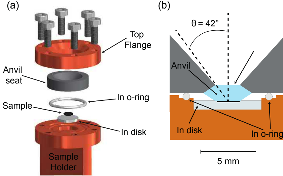
Figure A.2: Sample holder for MIR pump THz probe on \text{K}_3\text{C}_{60} at ambient pressure. In panel (a) all the mechanical components of the sample holder assembly are sketched. Panel (b) shows a side view of the sample compartment. The overall optical access is of 2\Theta \sim 85^\circ .
