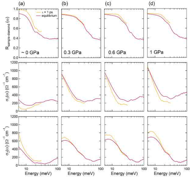
Figure 5.6: Pressure dependence of the transient optical properties of K_3C_{60} at 200K. Reflectivity (sample-diamond interface) and complex optical conductivity of K_3C_{60} measured at equilibrium (red) and 1 ps after photo-excitation (yellow), for different external pressures. All data were taken with the same pump fluence of 3 \text{ mJ/cm}^2 [24].
