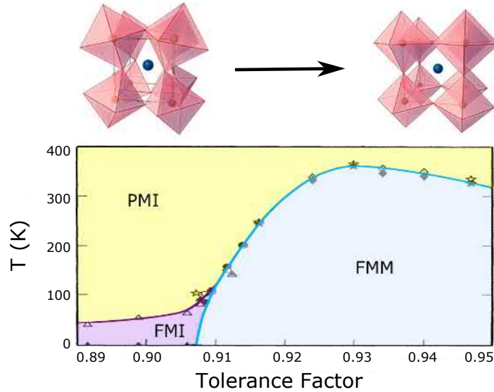
Figure 1.2: Phase diagram temperature vs tolerance factor for the system \text{A}_{0.7}\text{A}'_{0.3}\text{MnO}_3 , where A is a trivalent rare earth ion and A' is a divalent alkali earth ion. As the crystalline structure is perfectly cubic (tolerance factor approaches the unity) the system is metallic (FMM), while the distorted structure shows an insulating response (paramagnetic or ferromagnetic, PMI or FMI). Figure adapted from [31].
