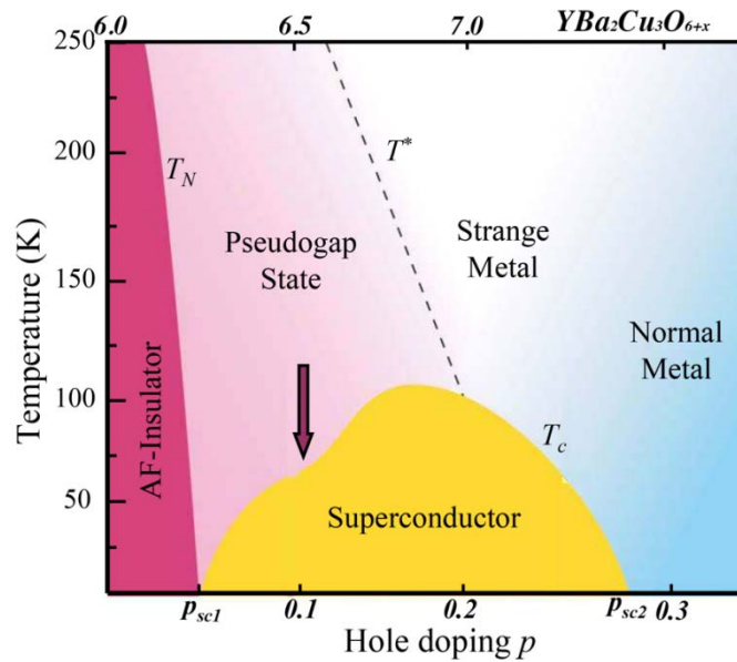
Figure 3.6. Phase diagram of the cuprate superconductors YBCO 6+x . The arrow indicates the YBCO 6.5 compound, which will be studied in Chapter 4. Adapted from Ref. [120].
