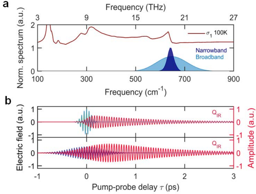
Figure C.4. (a) Equilibrium c -axis optical conductivity, \sigma_1(\omega) , of YB 2 Cu 3 O 6.5 at 100 K ( T > T_c , red solid line), along with the frequency spectra of THz probe (grey), broadband pump (light blue), and 19.2 THz narrowband pump (dark blue) pulses. (b) The amplitude of the 19.2-THz mode driven by 150 fs (upper) and 600 fs (lower) pump pulses with the same pulse energy.
