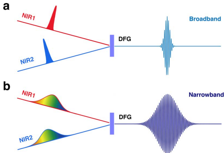
Figure 2.9. Schematics of the generation processes for (a) broadband and (b) narrowband THz pulses.
