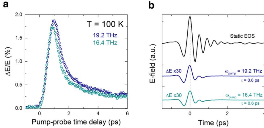
Figure 4.12. (a) Pump-induced changes at the peak of the THz probe electric field as a function of pump-probe time delay, measured in YBCO 6.5 at T = 100 K (below T_c ) for narrowband excitation at 16.4 THz and 19.2 THz excitations. (b) The static reflected probe electric field and corresponding pump-induced electric field changes for 19.2 THz and 16.4 THz at pump-probe delay \tau = 0.6 ps.
