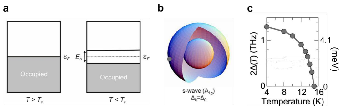
Figure 3.3. (a) Electronic state for a conventional superconductor above (left) and below (right) the transition temperature. The conduction band is occupied up to the Fermi level \varepsilon_F above T_c , while an energy gap opens around the Fermi surface below T_c . From Ref. [113]. (b) Gap function of s-wave symmetry, which is isotropic in the momentum space. From Ref. [113]. (c) Temperature dependence of the superconducting gap energy of a typical conventional superconductor NbN.
