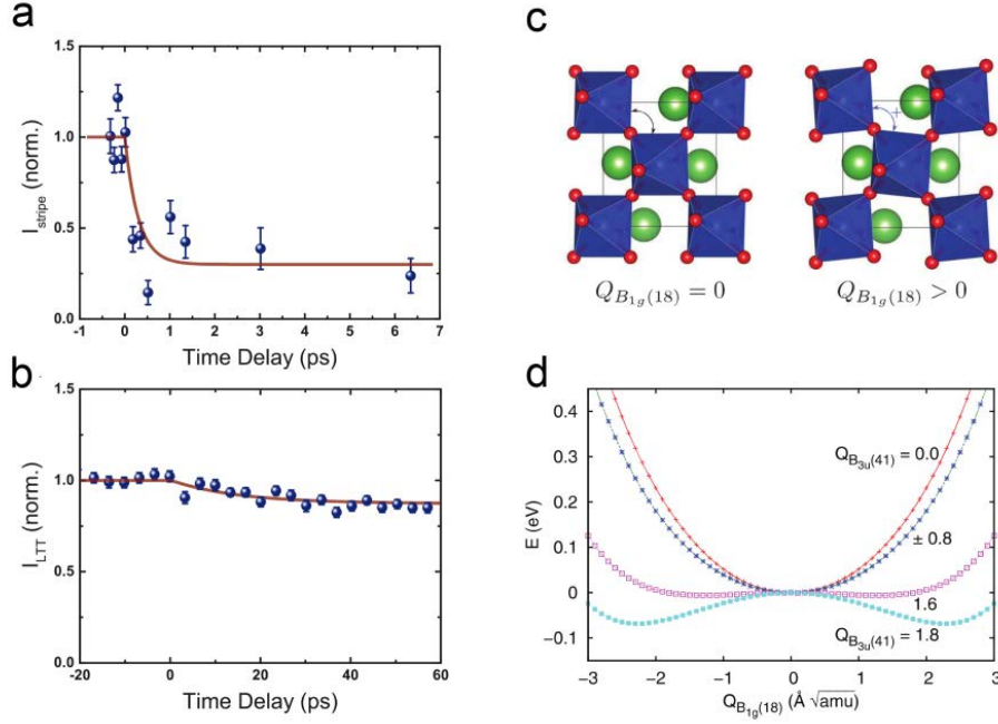
Figure 1.9. (a) Light-induced dynamic of the charge stripe order diffraction peak in \text{LBCO}_{1/8} . (b) Corresponding changes in the intensity of the diffraction peak associated with the LTT distortion in the same crystal under the same excitation conditions. Red lines: exponential fits with corresponding time constants. (c) Sketch of the atomic displacements of B_{1g} Raman mode in \text{La}_2\text{CuO}_4 . (d) Differential energy potential of the coupled Raman mode through quartic coupling. Taken from [5] [21].
