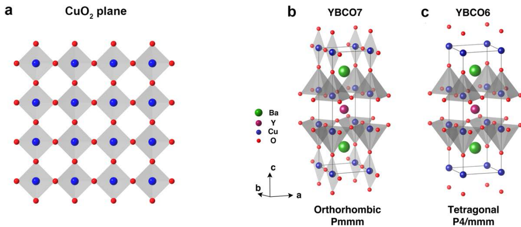
Figure 3.5. (a) Copper-oxygen plane in cuprates. (b) Orthorhombic structure of YBCO 7 (superconductor), which has Pmmm symmetry. (c) Tetragonal structure of YBCO 6 (insulator), which has P4/mmm symmetry. The octahedrons are highlighted in grey.
