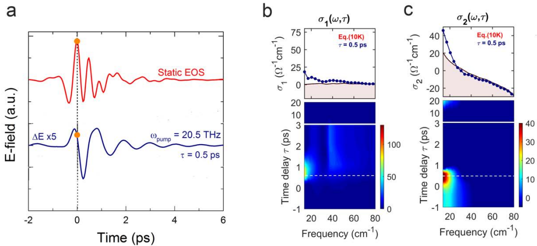
Figure 4.19. (a) Stationary reflected probe electric field and corresponding pump-induced electric field changes for 20.5 THz narrowband excitations at a pump-probe delay \tau = 0.5 ps. (b-c) Frequency- and time-delay-dependent pump-induced optical conductivity measured after narrowband excitation at 20.5 THz ( T = 10 K, below T_C ). The white dashed lines indicate the pump-probe time delay \tau = 0.5 ps.
