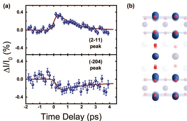
Figure 9. (a) Transient change in intensity of the (2\ \bar{1}\ 1) and the (\bar{2}\ 0\ 4) diffraction peaks in \text{YBa}_2\text{Cu}_3\text{O}_{6.5} , measured at 100 K following resonant excitation of the B_{1u} -symmetry apical oxygen mode. The red solid lines are fits as described in the text. (b) Corresponding transient crystal structure of \text{YBa}_2\text{Cu}_3\text{O}_{6.5} . The atomic displacements from the equilibrium structure are shaded.
