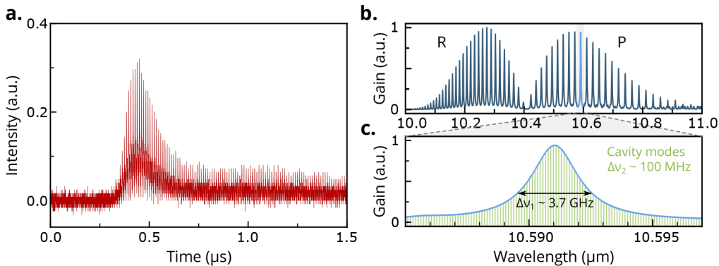
Fig. 2. Amplified spontaneous emission and multimode operation of the CO 2 laser oscillator.
