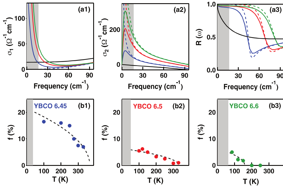
FIG. 10. (Color online) Results of the effective medium analysis. (a1)–(a3) Black curve: Optical properties of the unperturbed material. Blue curves: Extracted optical properties for the light-induced phase in YBCO 6.45 at 100 K [ \sigma_1(\omega) in panel (a1), \sigma_2(\omega) in panel (a2), reflectivity in panel (a3)]. Red curves: Extracted optical properties for the light-induced phase in YBCO 6.5 at 100 K. Green curves: Extracted optical properties for the light-induced phase in YBCO 6.6 at 100 K. Solid lines assume a solid that exhibits perfect transport for the 7 ps lifetime of the state. Dashed curves represent the optical properties of a perfect conductor with infinitely long lifetime. Both assumptions provide a satisfactory fit in our spectral range. (b1)–(b3) Fitted filling fraction as a function of temperature. The dashed curves are fits obtained with an empirical mean-field dependence of the type \propto \sqrt{1 - T/T_c} .
