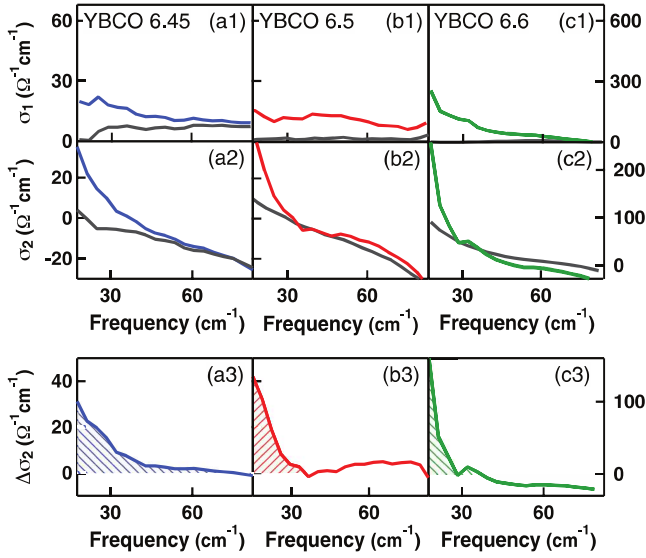
FIG. 3. (Color online) Below- T_c data. Optical properties of (a) YBCO 6.45, (b) YBCO 6.5, and (c) YBCO 6.6 in the superconducting state at 10 K base temperature. The gray lines describe the optical properties at equilibrium while the colored lines describe the response in the photostimulated state 0.8 ps after the excitation. The upper rows show \sigma_1 , the real part, and \sigma_2 , the imaginary part, of the complex optical response. The bottom row shows the photoinduced differential optical conductivity \Delta\sigma_2 between the optical properties in the photostimulated and the equilibrium state.
