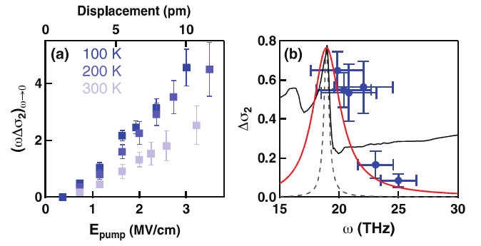
FIG. 6. (Color online) Fluence and wavelength dependence. (a) Size of the photoinduced enhancement \omega\Delta\sigma_2 for different pump fluences at 100 K, 200 K, and 300 K. The corresponding estimated displacement of the oxygen atoms (see Supplemental Material [24]) is shown in the top axis. (b) \Delta\sigma_2 at 1 THz plotted as a function of pump wavelength (blue dots) and measured at constant pump fluence. The horizontal bars indicate the pump spectral linewidth. The black line indicates equilibrium \sigma_1(\omega) . The resonant frequency of the apical oxygen mode is indicated in the dashed black curve, and in the red curve when convolved with the pump-pulse frequency bandwidth.
