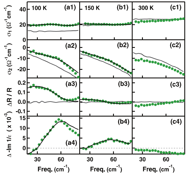
FIG. 8. (Color online) Optical properties YBCO 6.6 above T_c 0.8 ps time delay after excitation at (a) 100 K, (b) 150 K, and (c) 300 K. Green dots: Light-induced optical properties. Gray lines: Properties of the equilibrium state. Black lines: Effective medium fit for a transient conductor with \tau_s = 7 ps. (a1)–(c1) Real part of the optical conductivity \sigma_1(\omega) . (a2)–(c2) Imaginary part of the optical conductivity \sigma_2(\omega) . (a3)–(c3) Light-induced changes in reflectivity. Gray line: Change in reflectivity measured at negative time delays (no signal). (a4)–(c4) Light-induced changes in the energy loss function \Delta(-\text{Im}1/\epsilon) .
