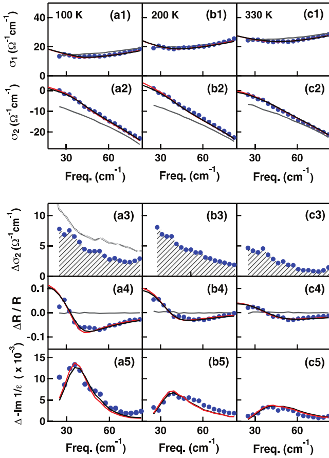
FIG. 5. (Color online) Optical properties YBCO 6.45 above T_c . 0.8 ps time delay after excitation at (a) 100 K, (b) 200 K, and (c) 330 K. Blue dots: Light-induced optical properties. Gray lines: Properties of the equilibrium state. Black lines: Effective medium fit for a transient conductor with \tau_s = 7 ps. Red lines: Effective medium fit for a perfect conductor with infinite lifetime. (a1)–(c1) Real part of the optical conductivity \sigma_1(\omega) . (a2)–(c2) Imaginary part of the optical conductivity \sigma_2(\omega) . (a3)–(c3) Differential changes in the imaginary conductivity \Delta\sigma_2(\omega, 1\text{ps}) = \sigma_2(\omega, 1\text{ps}) - \sigma_2^0(\omega) , where \sigma_2^0 is the equilibrium conductivity. Gray dotted curve: Change in imaginary conductivity \Delta\sigma_2(\omega, \Delta T) = \sigma_2^0(\omega, 10\text{K}) - \sigma_2^0(\omega, 60\text{K}) measured at equilibrium when cooling below T_c . (a4)–(c4) Light-induced changes in reflectivity. Gray line: Change in reflectivity measured at negative time delays (no signal). (a5)–(c5) Light-induced changes in the energy loss function \Delta(-\text{Im}1/\epsilon) .
