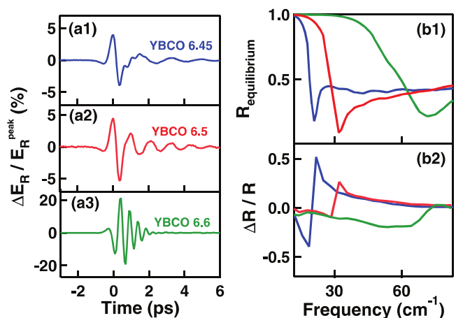
FIG. 2. (Color online) Below- T_c data. (a) Differential electric-field transient \Delta E_R(t, \tau)/E_R(t^{\text{peak}}) in YBCO 6.45 (blue), YBCO 6.5 (red), and YBCO 6.6 (green) excited with 20-THz pulses in the superconducting state at 20 K base temperature, measured with THz pulses polarized along the c axis (perpendicular to the superconducting planes). The response was measured at a time delay \tau = +0.8 ps after the 20-THz pump. (b1) Frequency-dependent reflectivities R_0 of YBCO 6.45, YBCO 6.5, and YBCO 6.6 measured at equilibrium along the c axis. Reflectivity edges of the Josephson plasma resonance are observed at \omega_{J,6.45} \sim 20 \text{ cm}^{-1} , \omega_{J,6.5} \sim 30 \text{ cm}^{-1} , and \omega_{J,6.6} \sim 60 \text{ cm}^{-1} . (b2) Corresponding frequency-dependent differential changes in the reflectivities \Delta R(\omega, 0.8 \text{ ps})/R_0 measured in (a1)–(a3) at positive time delays after the 20-THz pump. A shift of the Josephson plasma resonance is indicated.
