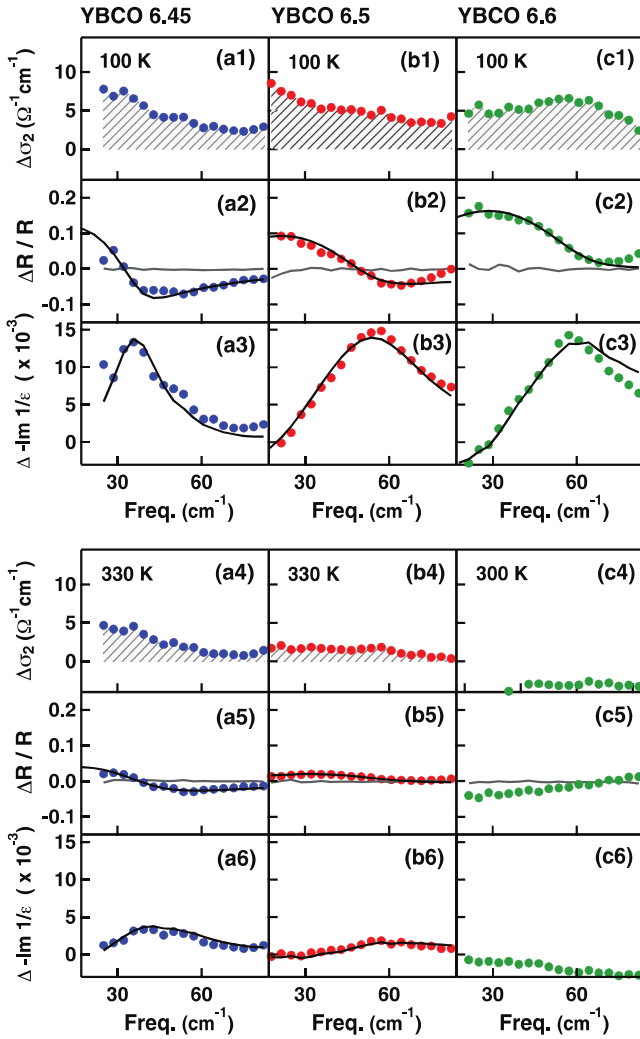
FIG. 9. (Color online) Doping-dependent transient optical properties of (a) YBCO 6.45, (b) YBCO 6.5, and (c) YBCO 6.6, 0.6 ps time delay after excitation (dots) at 100 K and high temperature. (a1)–(c1) Dots: Light-induced change in the optical conductivity \sigma_2(\omega) at 100 K. (a2)–(c2) Dots: Light-induced changes in reflectivity at 100 K. Black line: Effective medium fit. Gray line: Change in reflectivity measured at negative time delays (no signal). (a3)–(c3) Dots: Light-induced changes in the imaginary conductivity \Delta\sigma_2(\omega) at 330 K (YBCO 6.45 and YBCO 6.5) and 300 K (YBCO 6.6). (a4)–(c4) Dots: Light-induced changes in reflectivity at 330 K (YBCO 6.45 and YBCO 6.5) and 300 K (YBCO 6.6). Black line: Effective medium fit. Gray line: Change in reflectivity measured at negative time delays (no signal). (a5)–(c5) Dots: Light-induced changes in the energy loss function at 330 K (YBCO 6.45 and YBCO 6.5) and 300 K (YBCO 6.6). Black line: Effective medium fit.
