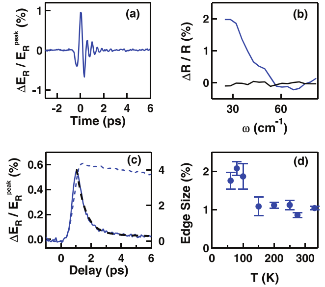
FIG. 4. (Color online) Above- T_c data. (a) Differential electric field transient \Delta E_R(t, \tau)/E_R(t^{\text{peak}}) in YBCO 6.45, excited with 20-THz pulses at 100 K base temperature. The response is measured with THz pulses polarized along the c axis (perpendicular to the superconducting planes) at a positive time delay ( \tau = +0.8 ps) after the 20-THz pump. (b) Frequency-dependent reflectivity changes measured along the c axis. The black line describes the equilibrium response at negative pump-probe time delays and the blue curve the response 0.8 ps excitation. A photoinduced reflectivity edge is observed at \omega_{J,6.45} \sim 43 \text{cm}^{-1} . (c) Delay dependence of the peak THz signal \Delta E_R(t^{\text{peak}}, \tau)/E_R(t^{\text{peak}}) as measured by scanning the pump-probe delay \tau for YBCO 6.45. \Delta E_R(t^{\text{peak}}, \tau) is proportional to the frequency-integrated effect. For comparison the blue dashed line describes the response below T_c . (d) The size of the photoinduced reflectivity edge as function of base temperature.
