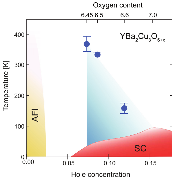
FIG. 11. (Color online) Schematic phase diagram of YBCO, where the equilibrium phases (superconducting and antiferromagnetic), as well as the nonequilibrium phase discussed in this paper, are displayed. The blue dots are the T_c values extracted from the fits in Figs. 10(b1)–10(b3).
