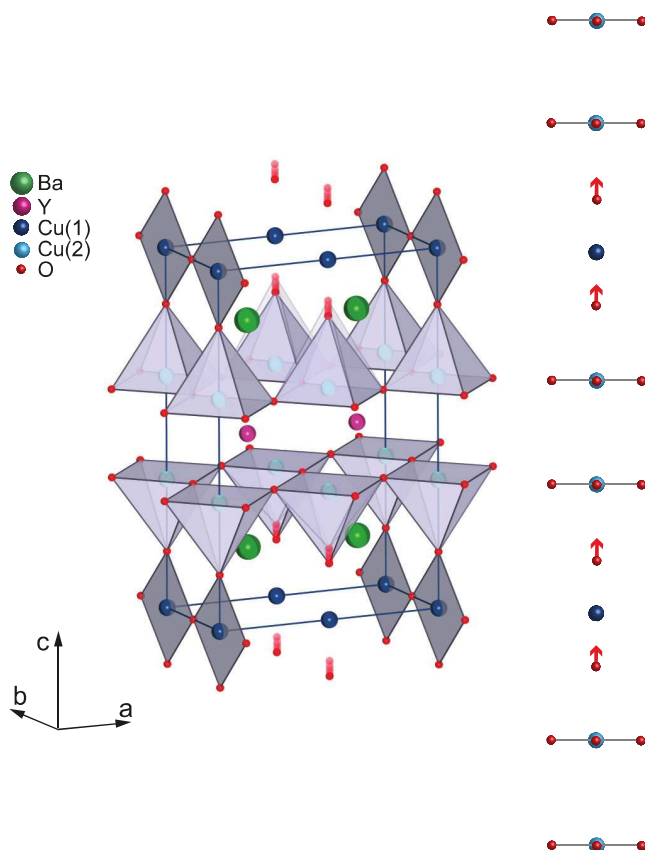
FIG. 1. (Color online) Structure of \text{YBa}_2\text{Cu}_3\text{O}_{6.5} and lattice distortion for the 20-THz mode. Two conducting \text{CuO}_2 planes [Cu(2), and O in the ab plane] are separated by Y atoms (pink) and form a bilayer unit. Ba atoms (green) and the \text{CuO}_4 ribbons [Cu(1), and O in the bc plane] separate bilayer units [25]. The excitation of the infrared-active B_{1u} mode at 20-THz frequency modulates only the displacement of the apical oxygen atoms along the c direction [26].
